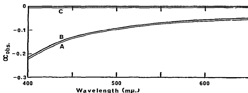
Fig. 2. The Optical and Pfeiffer rotatory dispersion of the L-[Ni( o -phen) 3 ] ++ ion. A: The ORD of 5.4 \times 10^{-4} \text{ M} . L-[Ni( o -phen) 3 ] ++ in water (1 cm cell, 25^\circ \text{ C} ). B: The ORD of 0.05 \text{ M} D,L-[Ni( o -phen) 3 ] ++ + 0.05 \text{ M} levo -malic acid in water (1 cm cell, 25^\circ \text{ C} ). C: The ORD of 0.05 \text{ M} levo -malic acid in water (1 cm cell, 25^\circ \text{ C} ).
